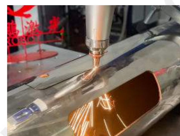
3D Cutting of Pipes
